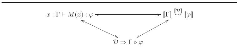
Figure 2. Curry–Howard–Lambek correspondence
