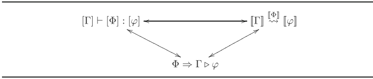
Figure 3. Constructions-as-Realizers-as-Arrows Correspondence
